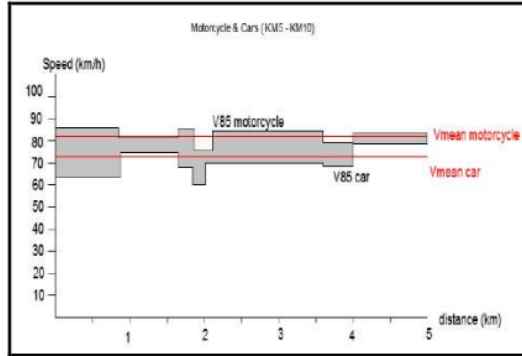
Fig 9 - Integrated speed profiles cars - motorcycles
